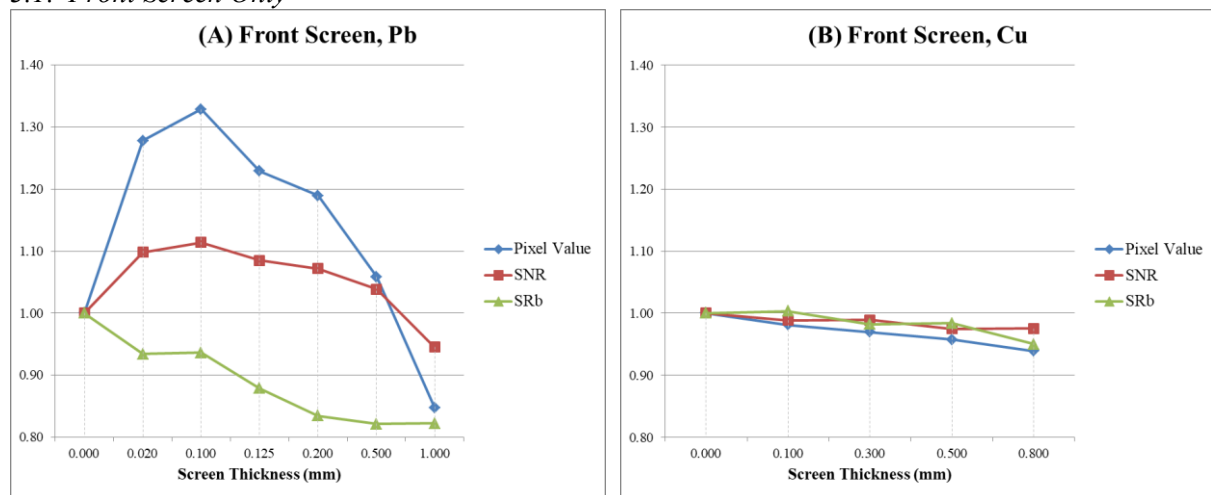
Figure 3. Effects of lead (A) and copper (B) front screen thickness on image quality.
